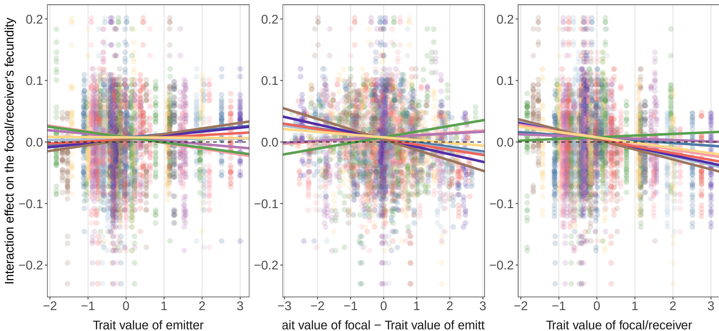
INTERspecific interactions with low density of emitter individuals
